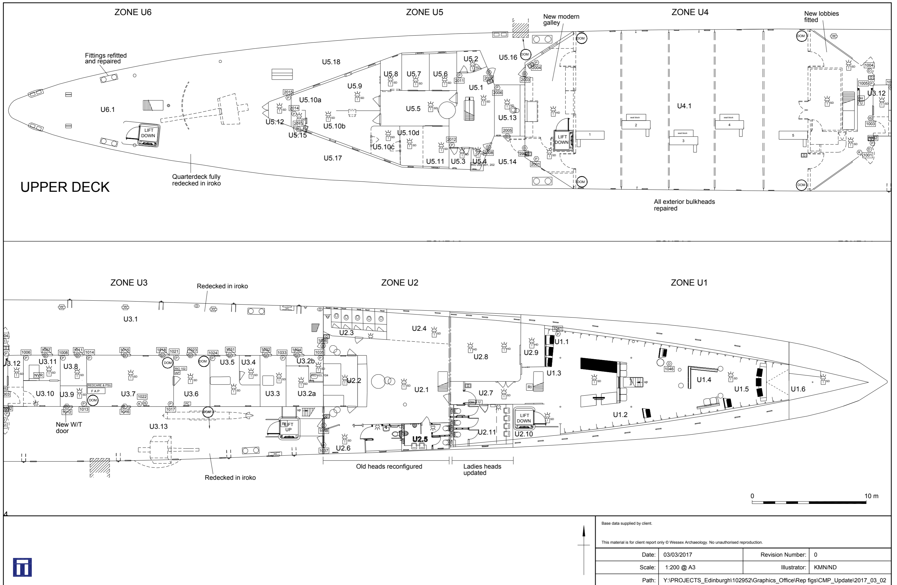
Updated Upper Deck Plan of HMS Caroline following refit
