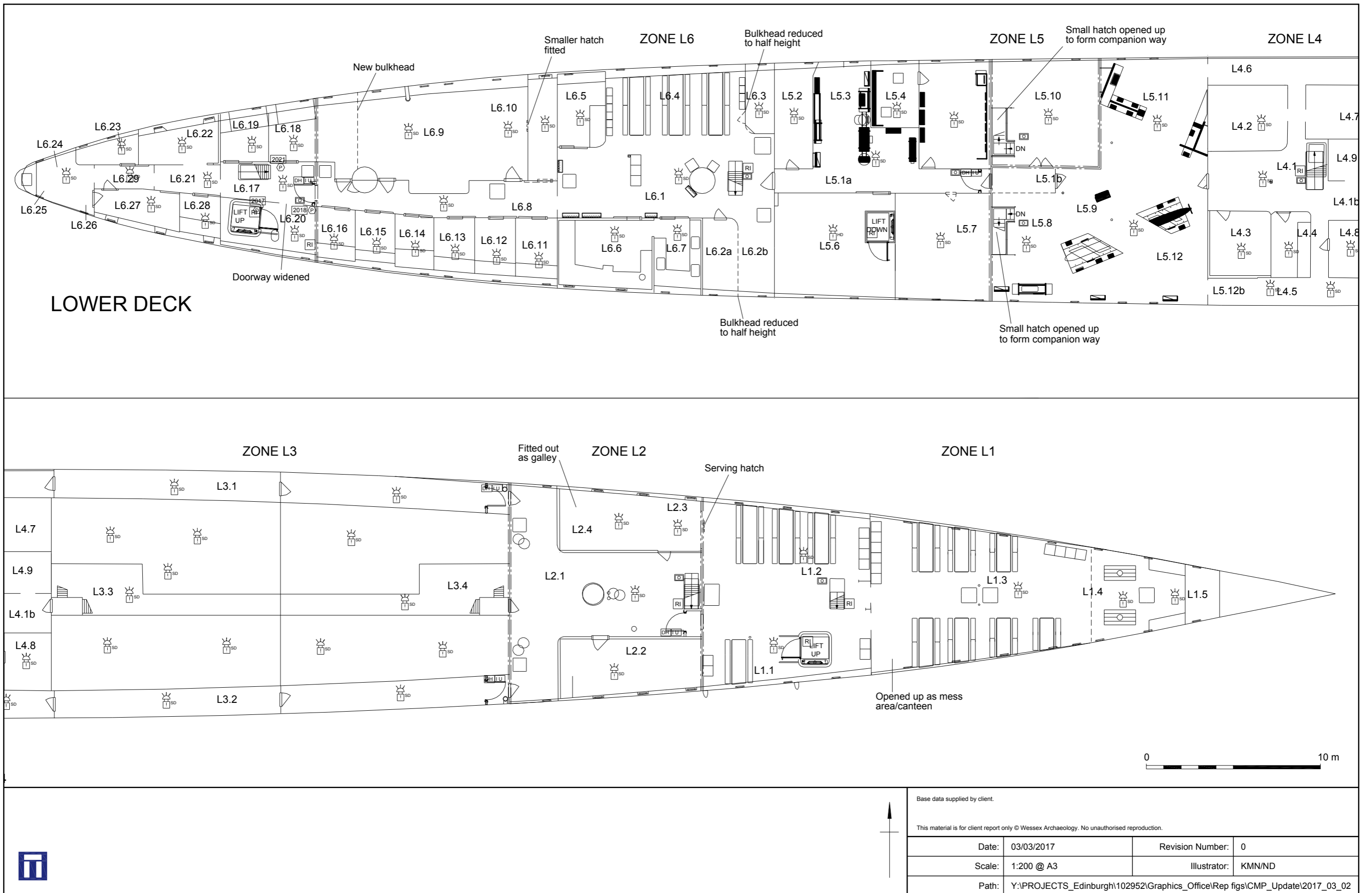
Updated Lower Deck Plan of HMS Caroline following refit
