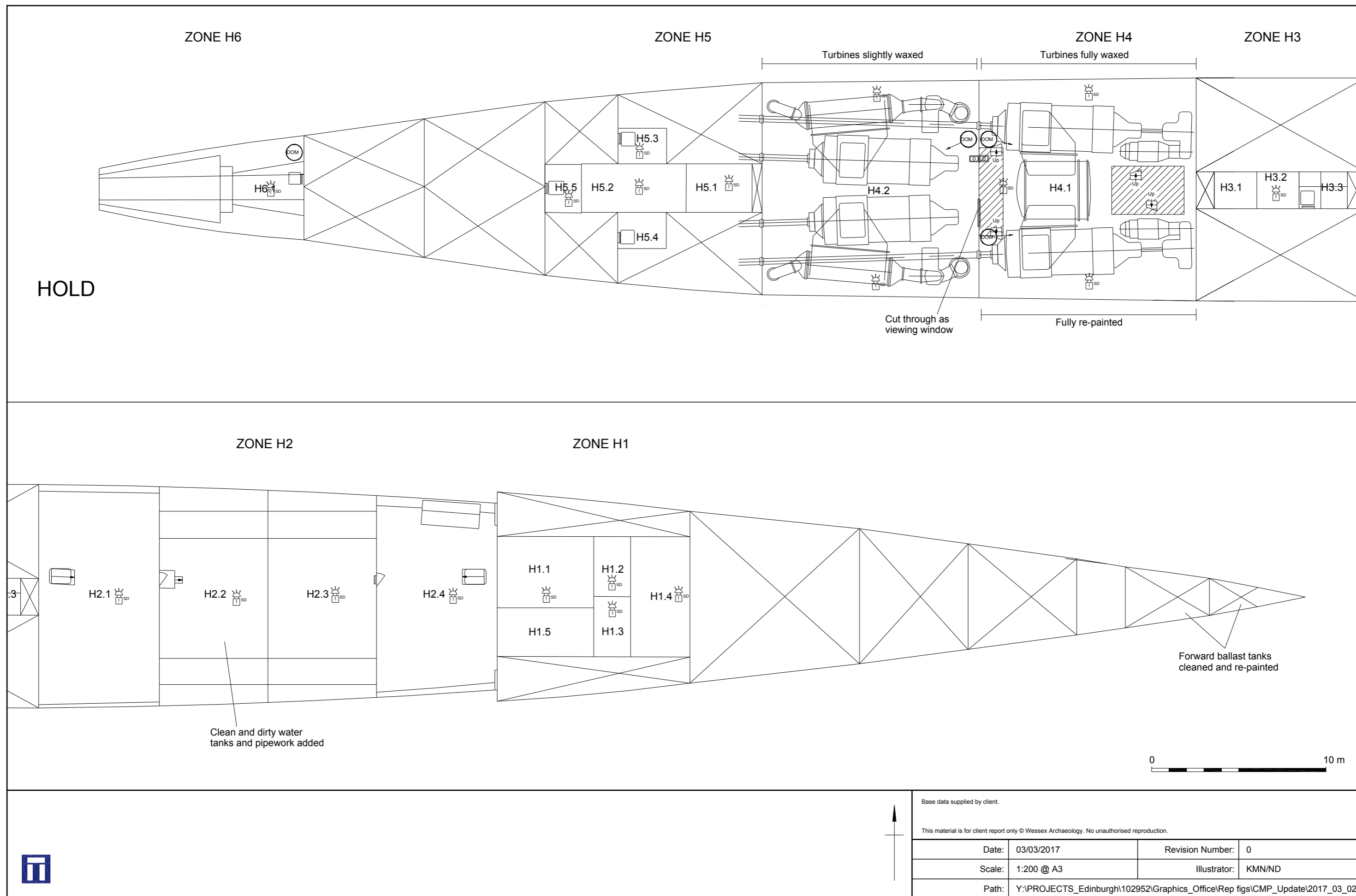
Updated Hold Plan of HMS Caroline following refit
